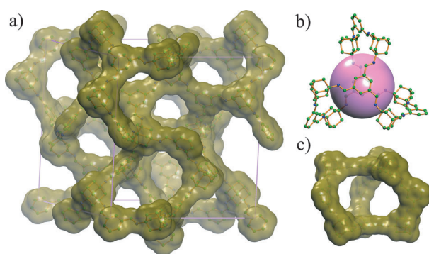
Figure 2. Extended structure of BF-COF-1. a) Atomic connectivity in BF-COF-1 with atom surfaces in olive green. Carbon and nitrogen are represented as green and blue spheres, respectively. b) A microporous cavity (pink sphere) with a diameter of 7.8 Å in BF-COF-1. c) Rectangular windows with a diameter of 7.8 \times 11.3 \text{ Å}^2 in BF-COF-1.
